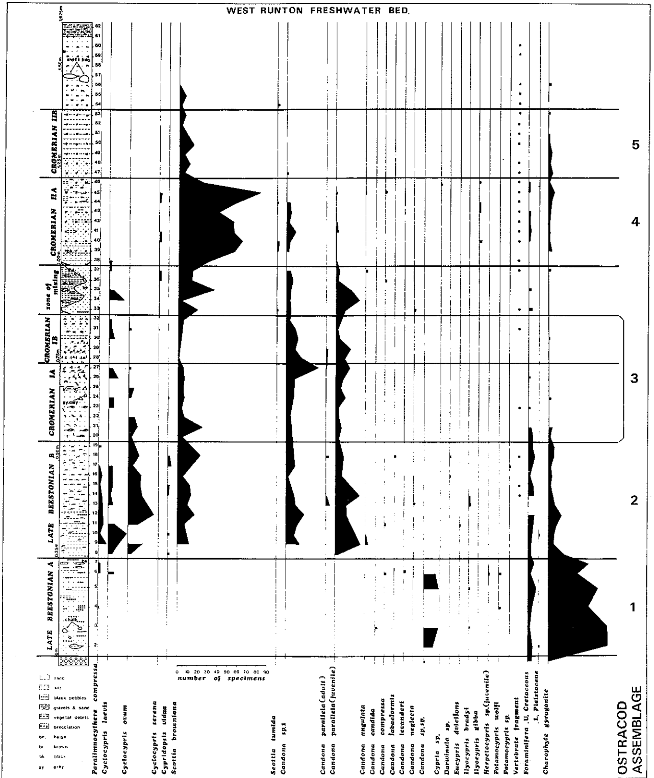
TEXT-FIG. 1. Distribution of the ostracods recorded at West Runton. Note that the ostracod assemblages correspond to the pollen assemblage zones studied by West (in press). Sample numbers are to be preceded with the letters CR.
