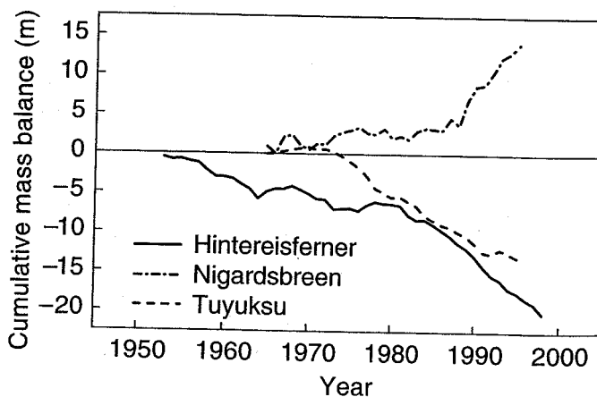
Figure 11.2: Cumulative mass balance for 1952-1998 for three glaciers in different climatic regimes: Hintereisferner (Austrian Alps), Nigardsbreen (Norway), Tuyuksu (Tien Shan, Kazakhstan).
