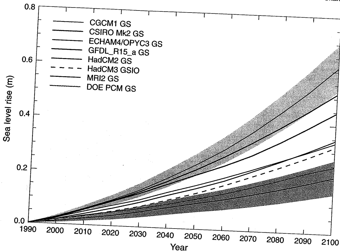
Figure 11.11: Global average sea level rise 1990 to 2100 for the IS92a scenario, including the direct effect of sulphate aerosols. Thermal expansion and land ice changes were calculated from AOGCM experiments, and contributions from changes in permafrost, the effect of sediment deposition and the long-term adjustment of the ice sheets to past climate change were added. For the models that project the largest (CGCM1) and the smallest (MRI2) sea level change, the shaded region shows the bounds of uncertainty associated with land ice changes, permafrost changes and sediment deposition. Uncertainties are not shown for the other models, but can be found in Table 11.14. The outermost limits of the shaded regions indicate our range of uncertainty in projecting sea level change for the IS92a scenario.
