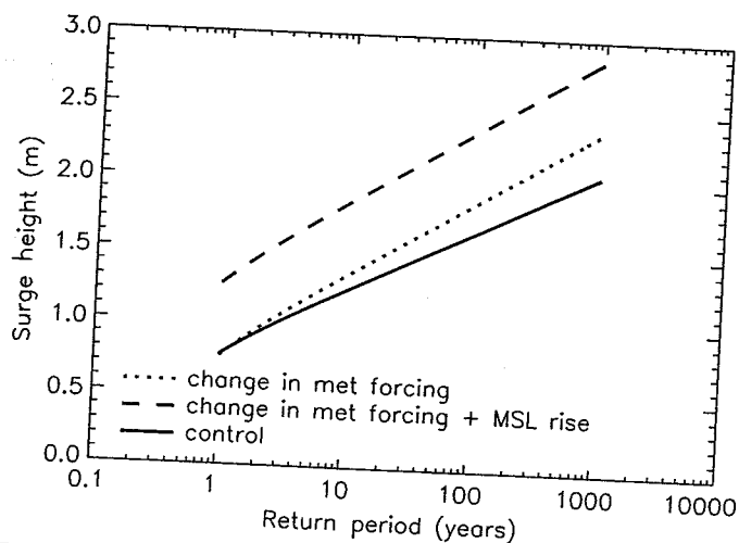
Figure 11.14: Frequency of extreme water level, expressed as return period, from a storm surge model for present day conditions (control) and the projected climate around 2100 for Immingham on the east coast of England, showing changes resulting from mean sea level rise and changes in meteorological forcing. The water level is relative to the sum of present day mean sea level and the tide at the time of the surge. (From Lowe et al. , 2001.)
