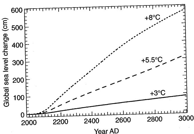
Figure 11.16: Response of the Greenland Ice Sheet to three climatic warming scenarios during the third millennium expressed in equivalent changes of global sea level. The curve labels refer to the mean annual temperature rise over Greenland by 3000 AD as predicted by a two-dimensional climate and ocean model forced by greenhouse gas concentration rises until 2130 AD and kept constant after that. (From Huybrechts and De Wolde, 1999.) Note that projected temperatures over Greenland are generally greater than globally averaged temperatures (by a factor of 1.2 to 3.1 for the range of AOGCMs used in this chapter). See Table 11.13 and Chapter 9, Fig 9.10c.
