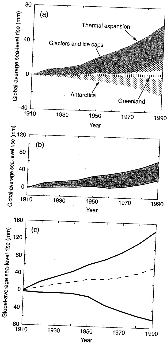
Figure 11.10: Estimated sea level rise from 1910 to 1990. (a) The thermal expansion, glacier and ice cap, Greenland and Antarctic contributions resulting from climate change in the 20th century calculated from a range of AOGCMs. Note that uncertainties in land ice calculations have not been included. (b) The mid-range and upper and lower bounds for the computed response of sea level to climate change (the sum of the terms in (a) plus the contribution from permafrost). These curves represent our estimate of the impact of anthropogenic climate change on sea level during the 20th century. (c) The mid-range and upper and lower bounds for the computed sea level change (the sum of all terms in (a) with the addition of changes in permafrost, the effect of sediment deposition, the long-term adjustment of the ice-sheets to past climate change and the terrestrial storage terms).
