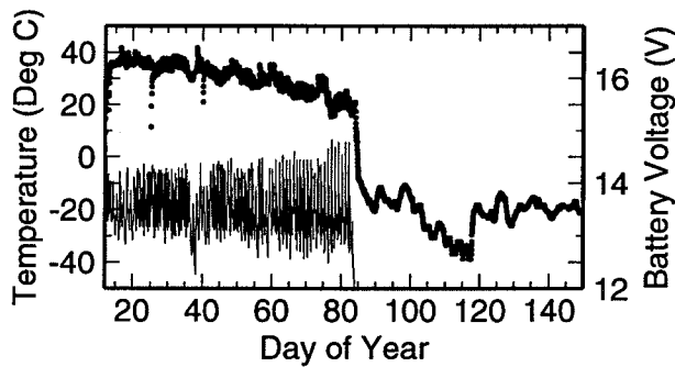
Fig. 3. Internal housing temperature (circles) and battery voltage (thin line) for the 1998 solar-powered GPS equipment. The equipment ceased operating on day 084 because of a lack of power. The internal temperature rapidly cooled then tracked the external air temperature. Temperature drops on days 25 and 40 were caused by the opening of the suitcase in order retrieve GPS data from the computer.
